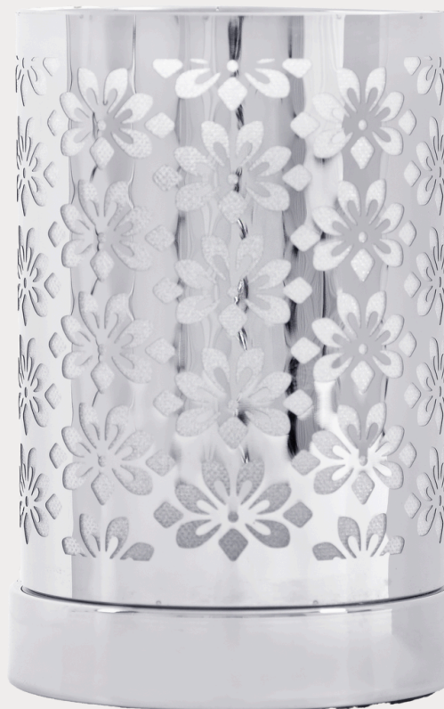
Bellatrix
