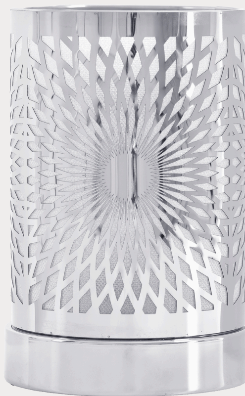
Sirius
